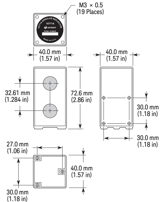
Keysight 10771A Angular Reflector Net Wt: 650g (1.5 lb)
