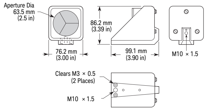
Keysight 10776-67001 Straightness Retroreflector Net Wt: 374g (0.82 lb)
