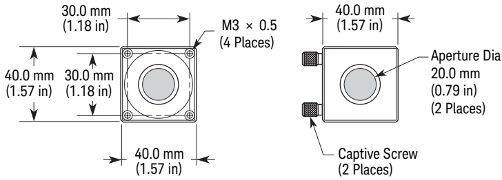
Keysight 10772A Tuning Mirror Net Wt: 510g (1.2 lb) w/Mount
