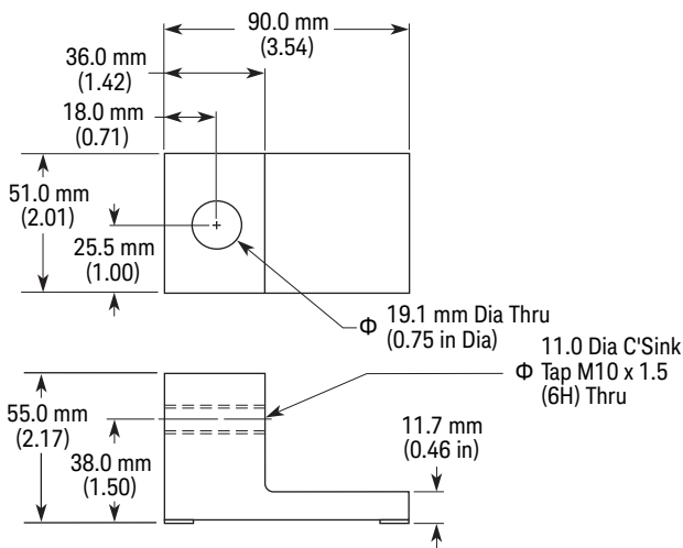
Keysight 10776A Straightness Mount
