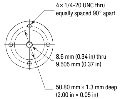
Flanged Shaft
