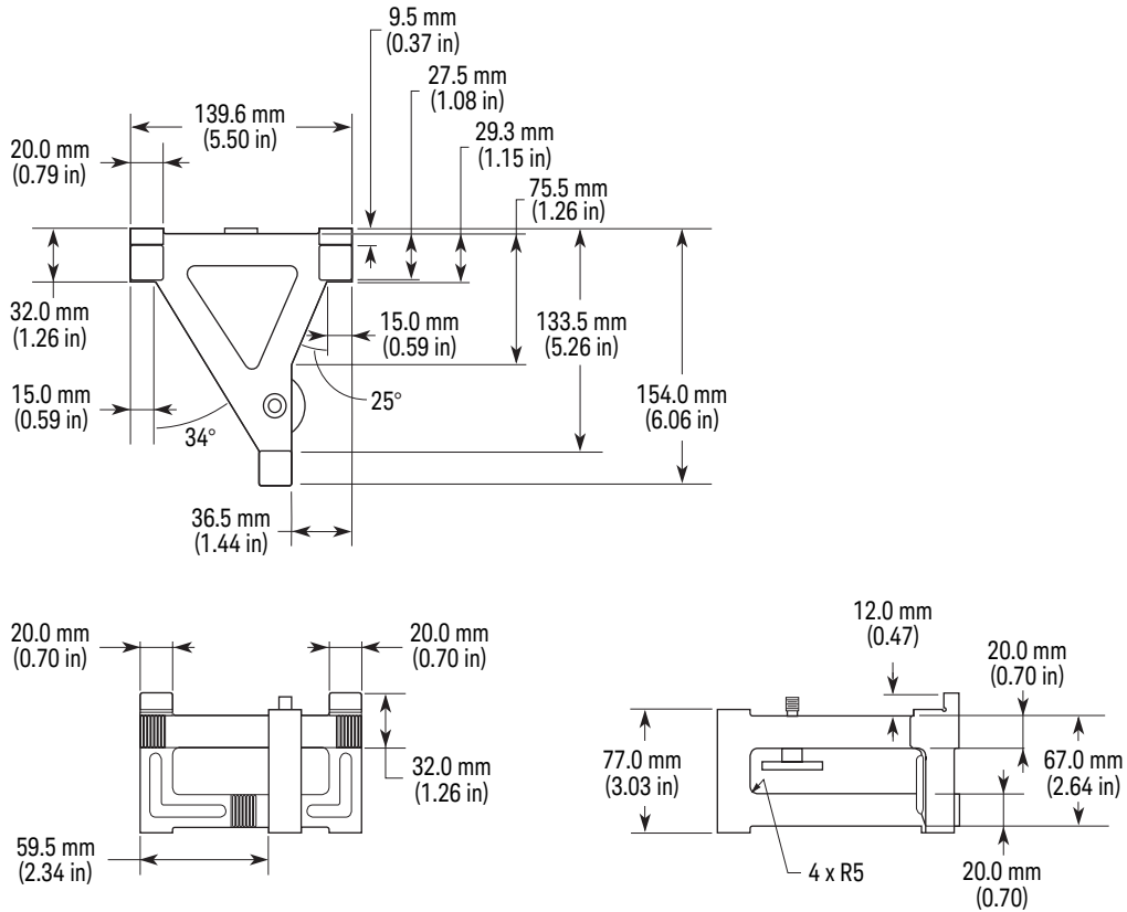
Keysight 10777-2007 Optical Square Base
